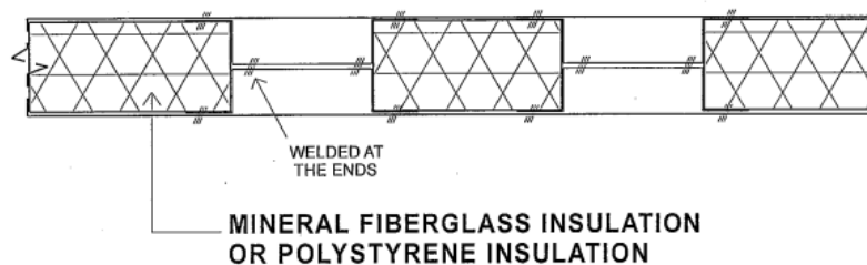
STEEL RIBBED SECTION
